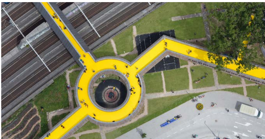
The Luchtsingel footbridge, in Rotterdam, is a crowd funded project connecting the city's disconnected areas.
